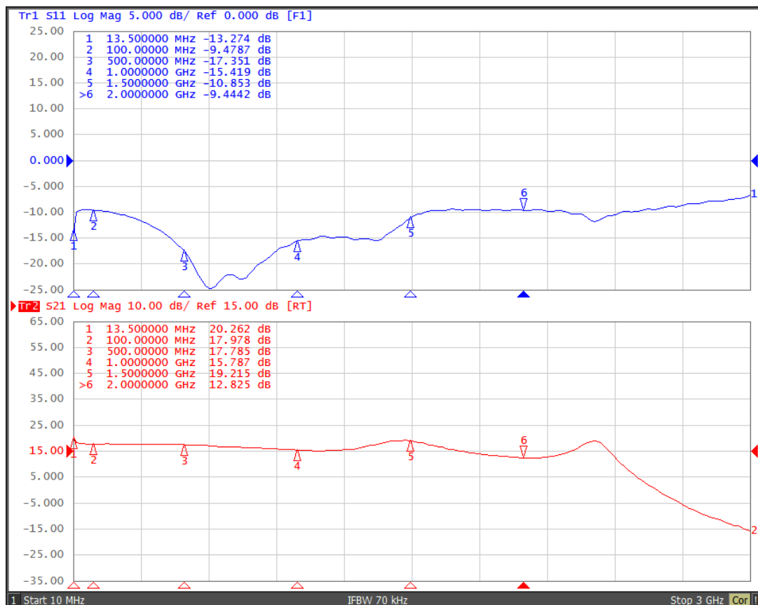
Figure 1. Network analyzer output S11/S21 (Pin=0dBm)
