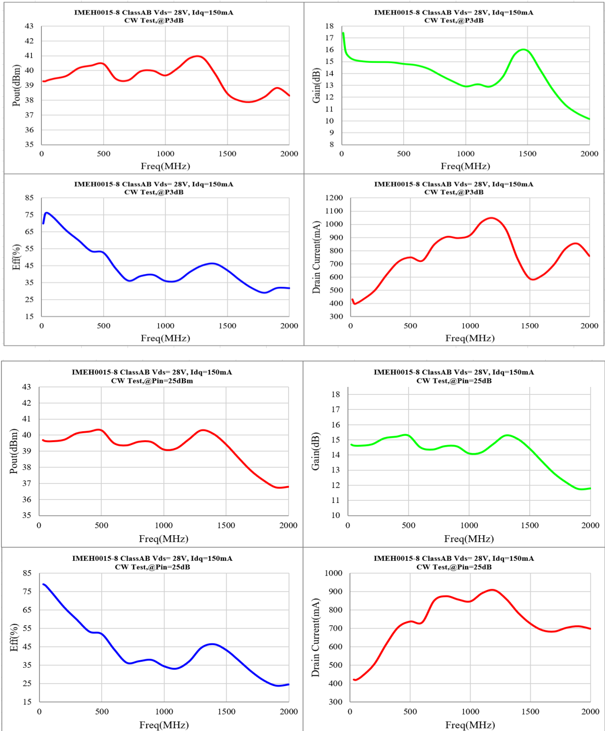
Figure. Power Gain and, efficiency and Pout @Pin=25dBm ,and P3dB vs. Frequency
