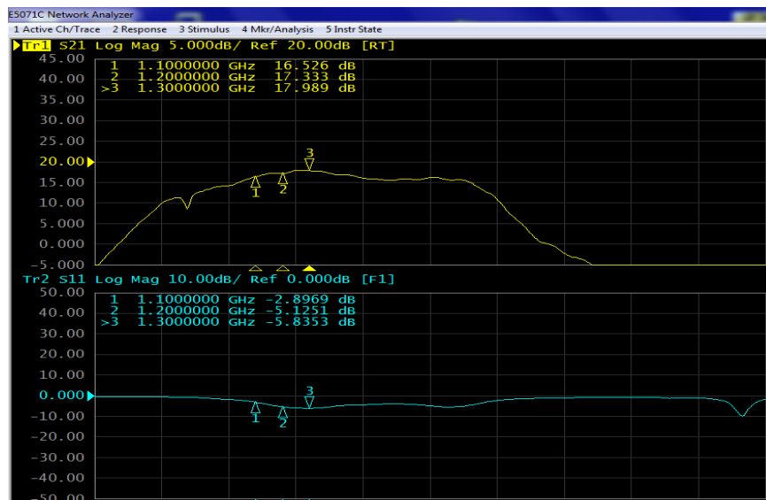
Figure 3: Network analyzer output, S11 and S21 ( VDS=28V VGS=-2.61V IDQ=500mA)
