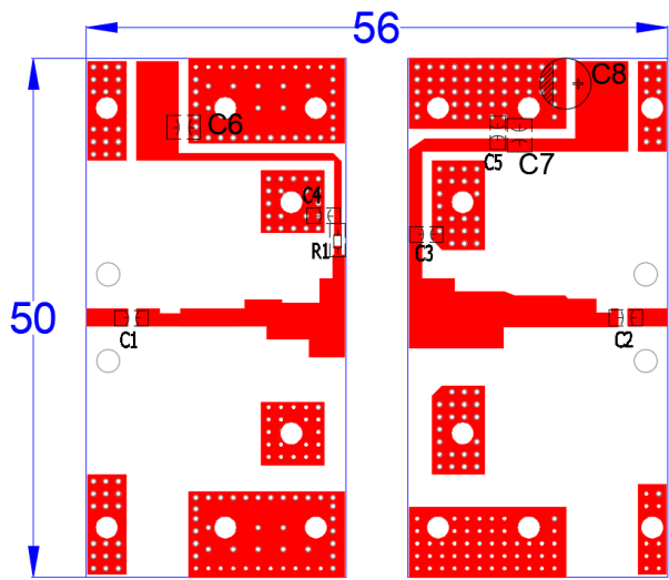
Figure 1. Test Circuit Component Layout (4-8GHz)
