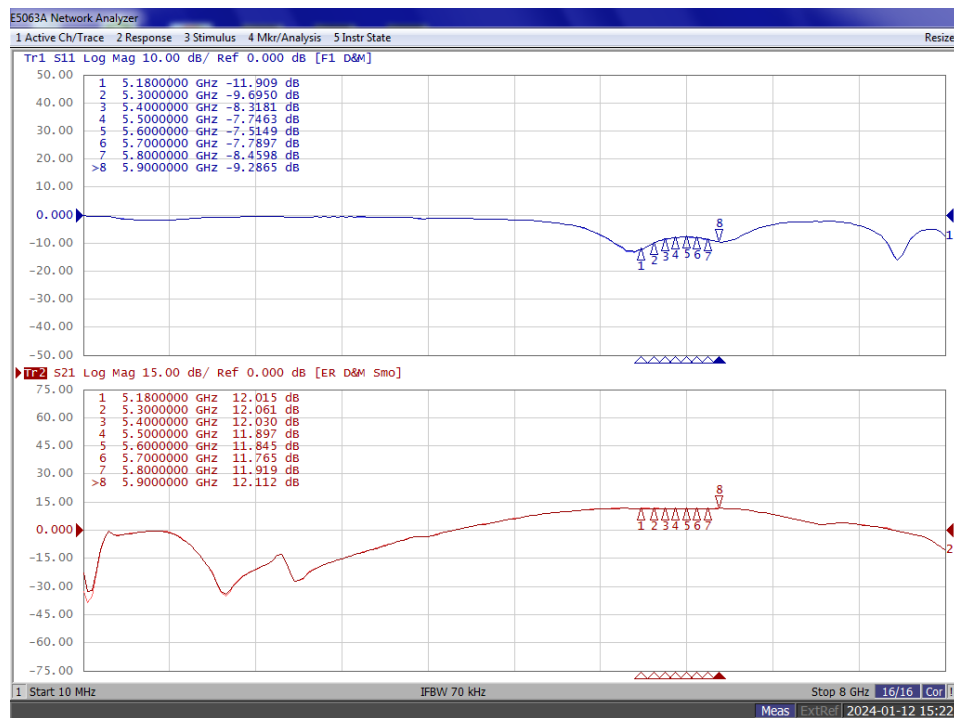
Figure 4: Small signal gain and return loss Vs Frequency Vds=28V, Idq=100mA, input power=0dBm
