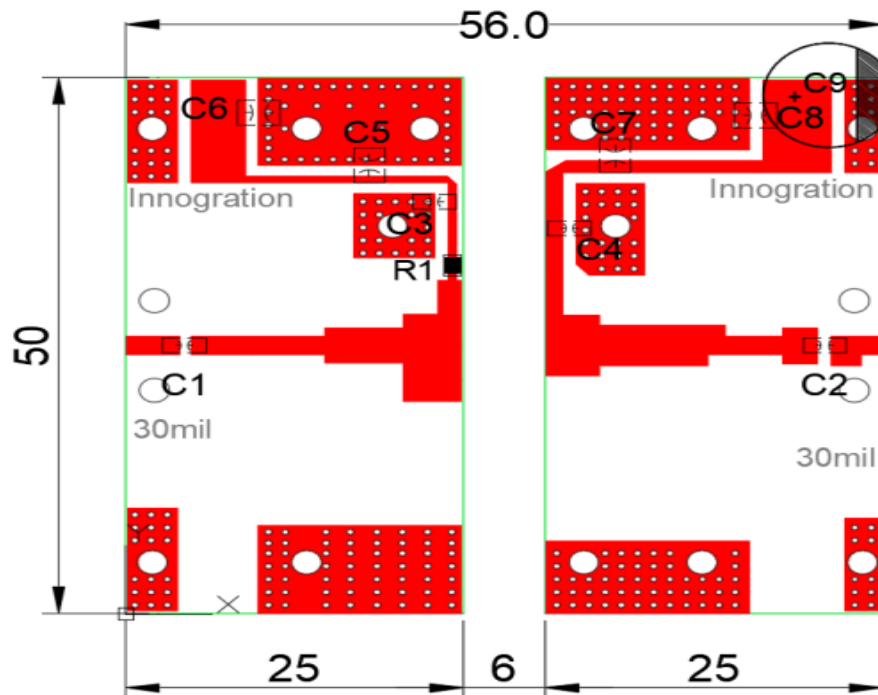
Figure 3: Picture and Bill of materials of 5.7-5.9GHz wide band application circuit (Layout Gerber file upon request)
