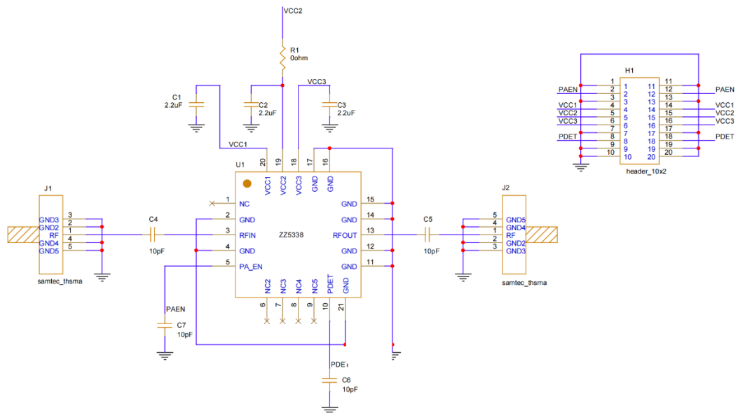
Figure 4: Application Circuit Schematic
