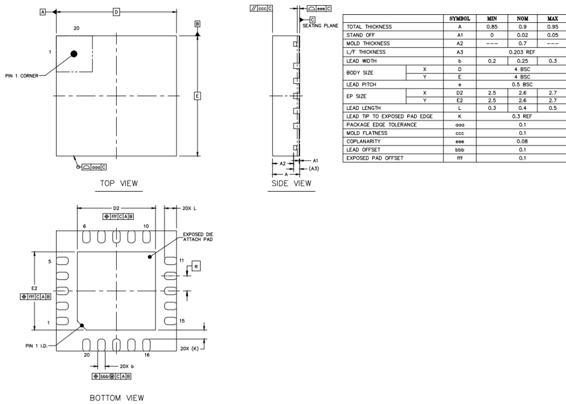
Figure 5: Package Outline
