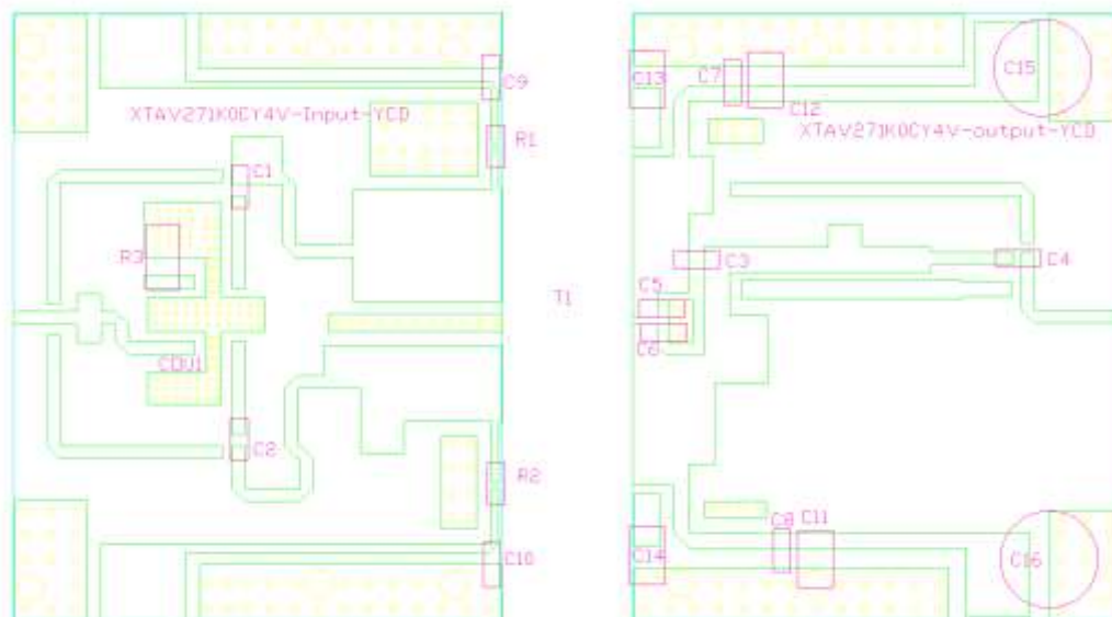
Figure 3: Picture of application board Doherty circuit for 2.5-2.7GHz
